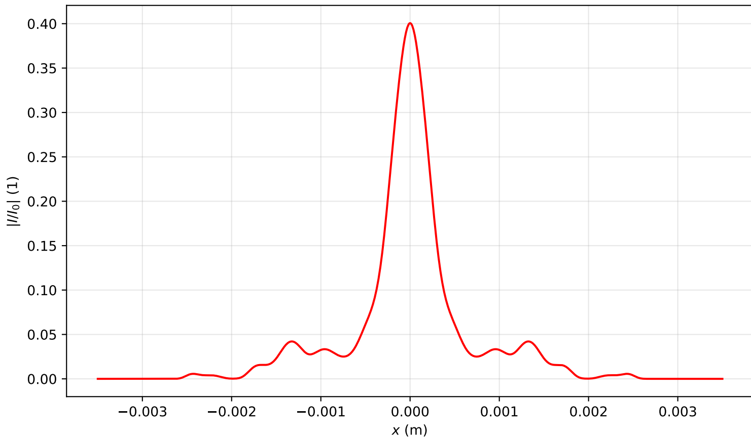
Intensity profile I(x, y = 0, z = 3.344)/I_0 , P_{in}=5.0P_{cr} , artificial time
